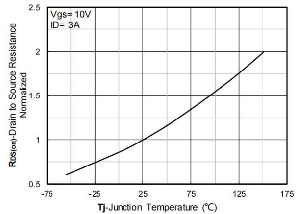
Figure 6. Normalized On-Resistance
