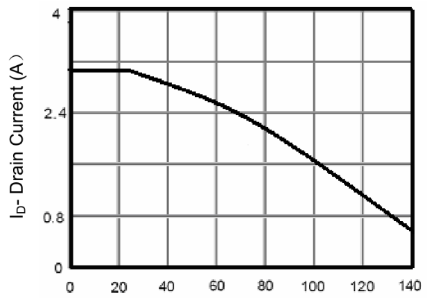
Figure 4 Drain Current
