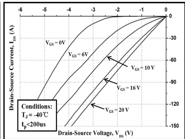
Figure 12. 3rd Quadrant Characteristic at -40 °C
