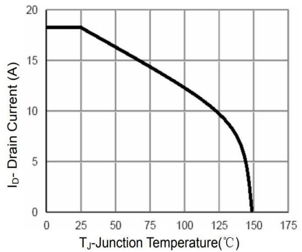
Figure 10 Current De-rating
