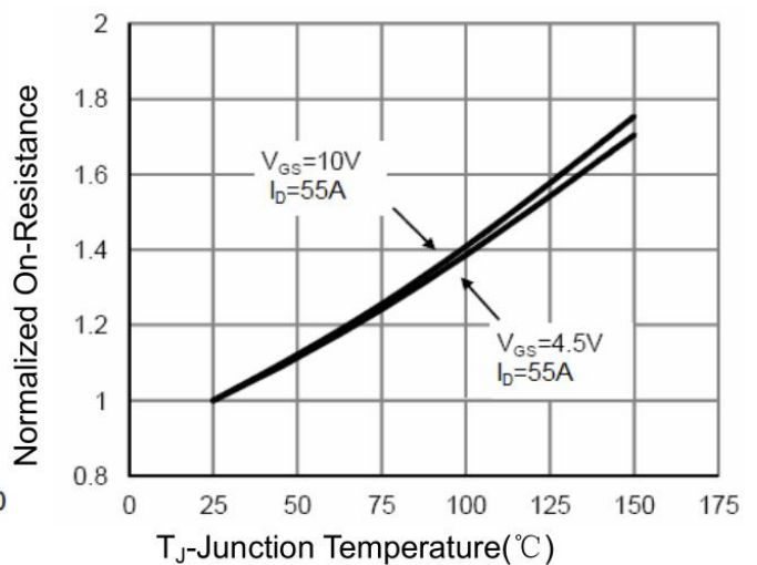
Figure 4 Rdson-Junction Temperature
