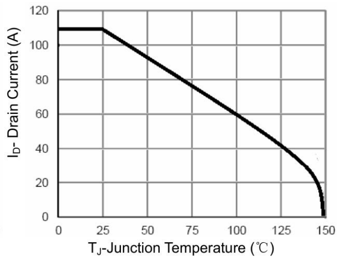
Figure 10 Current De-rating
