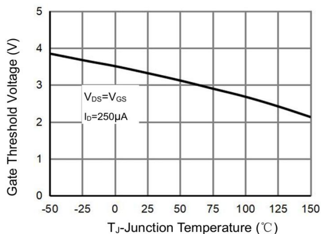
Figure 9 V_{GS(th)} -Junction Temperature
