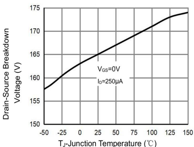
Figure 12 BV_{DS} -Junction Temperature
