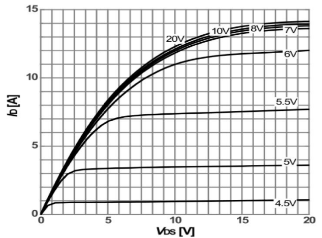
Figure 4: Typ. output characteristics
