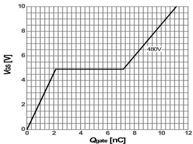
Figure8: Type. gate charge
