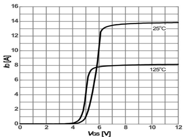
Figure7: Type. transfer characteristics
