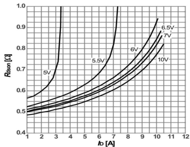
Figure 5: Typ. drain-source on-state resistance
