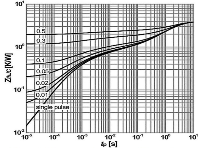
Figure 2: Max. transient thermal impedance
