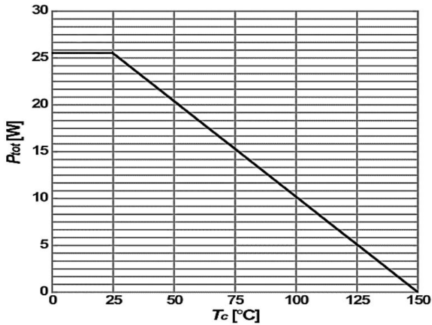
Figure 1: Power dissipation
