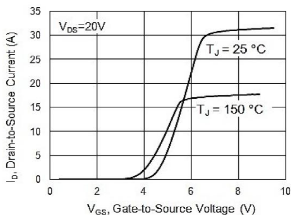
Figure8: Transfer characteristics
