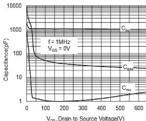
Figure4: Capacitance Characteristics
