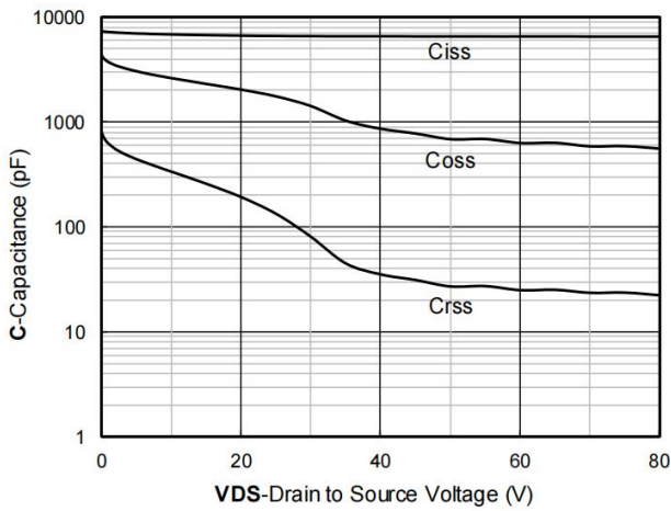
Figure 3. Capacitance Characteristics
