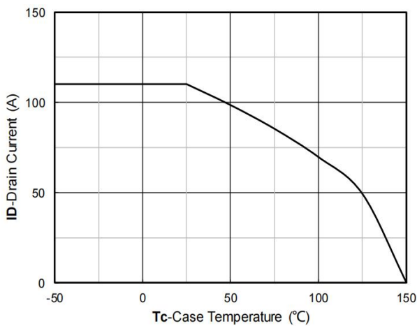
Figure 11. Current dissipation
