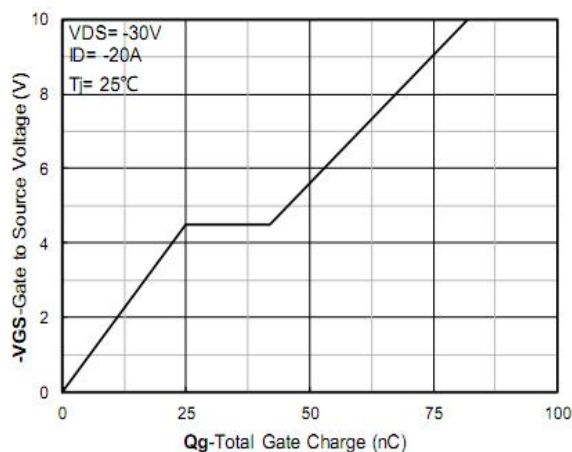
Figure 4. Gate Charge
