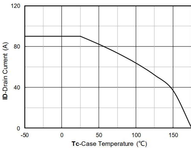
Figure 11. Current dissipation
