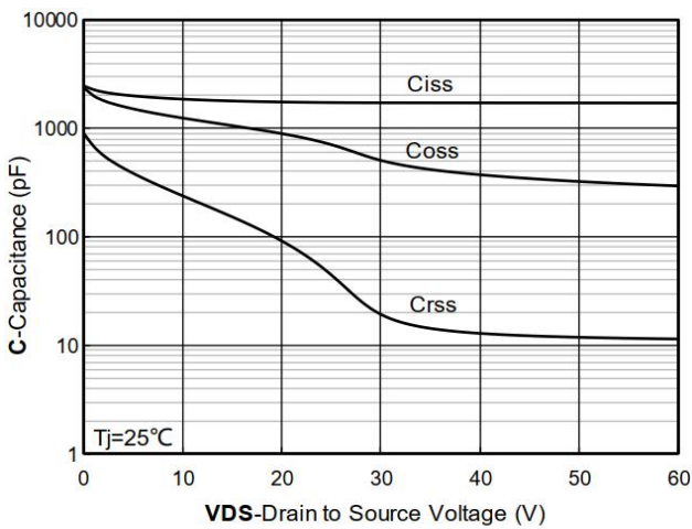
Figure 3. Capacitance Characteristics
