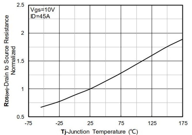
Figure 6. Normalized On-Resistance
