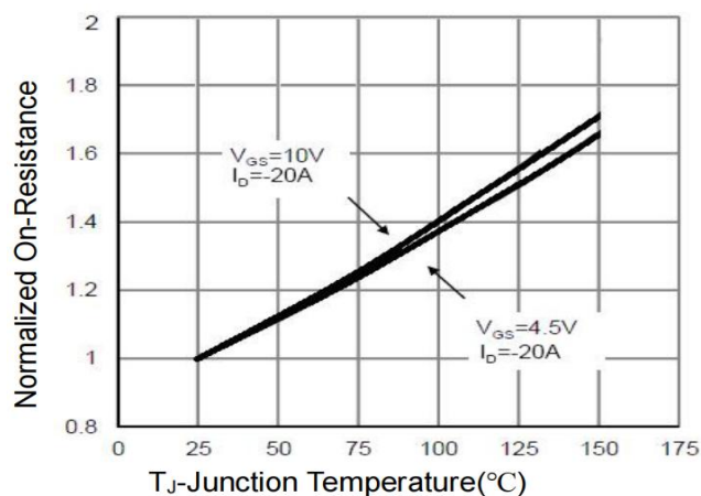
Figure 4 Rdson-Junction Temperature
