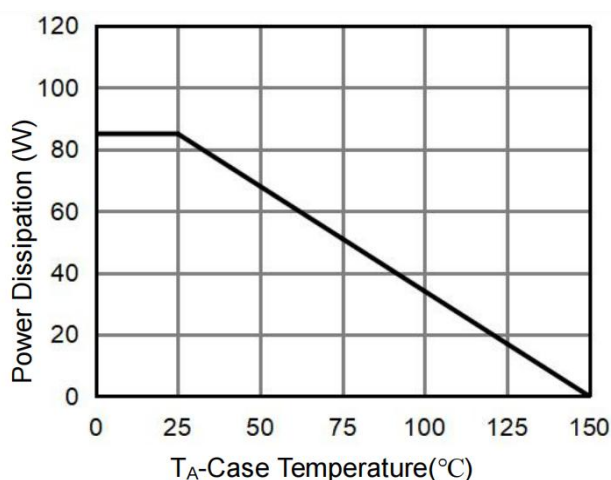
Figure 9 Power De-rating
