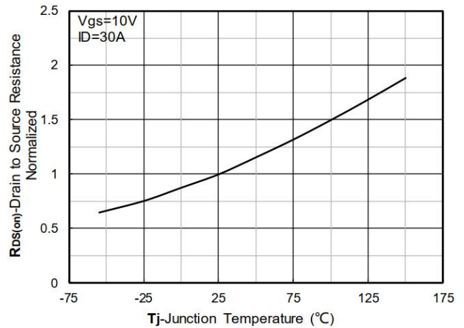
Figure 6. Normalized On-Resistance
