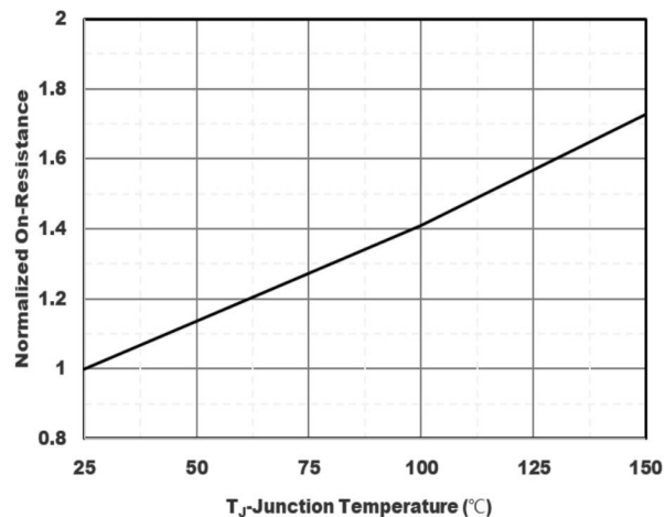
Figure6. Normalized On-Resistance
