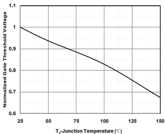
Figure 7. Normalized Gate Threshold Voltage
