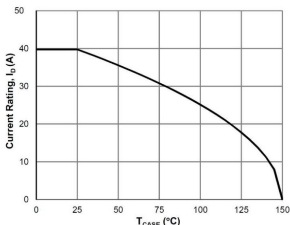
Current De-rating
