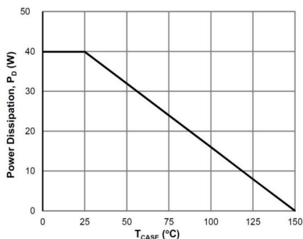
Power De-rating
