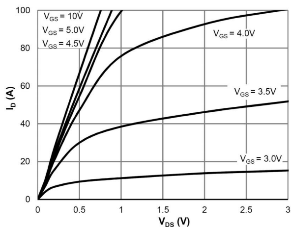
Saturation Characteristics
