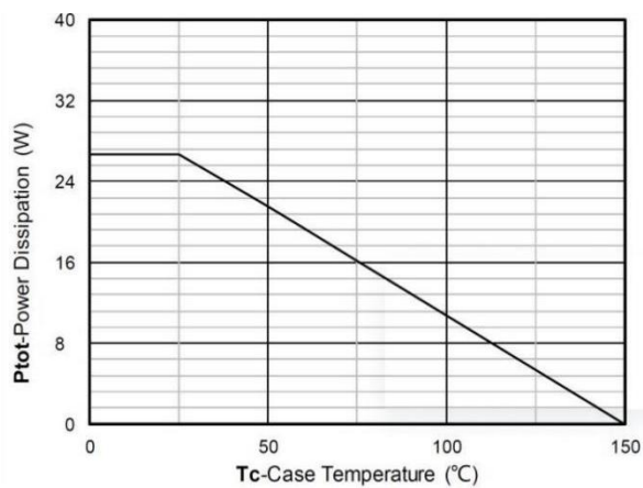
Power dissipation
