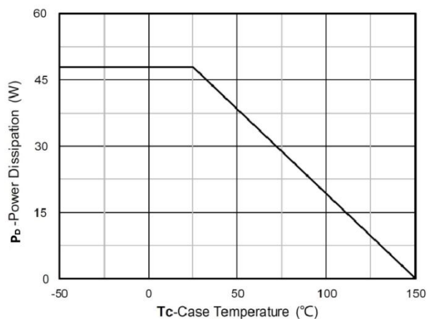
Power dissipation
