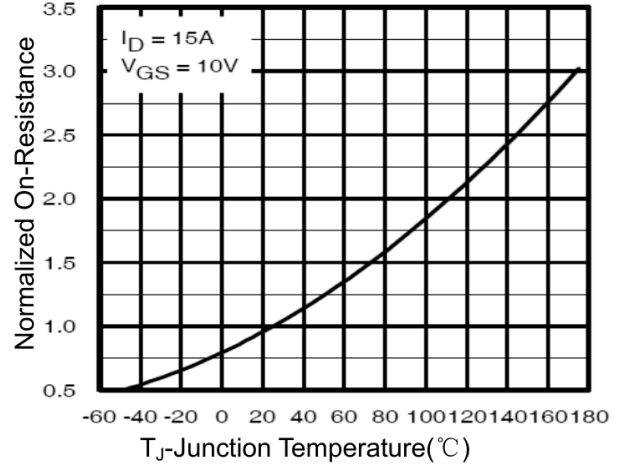
Figure 4 Rdson-Junction Temperature
