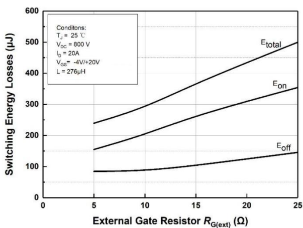
Figure 21. Clamped Inductive Switching
