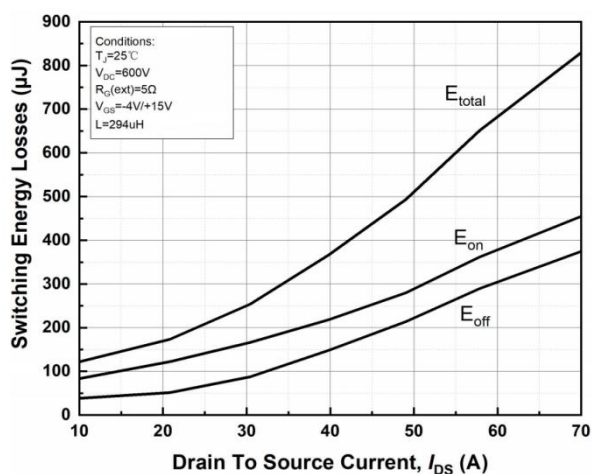
Figure 19. Clamped Inductive Switching Energy vs. Drain Current ( V_{DD} = 600\text{V} )
