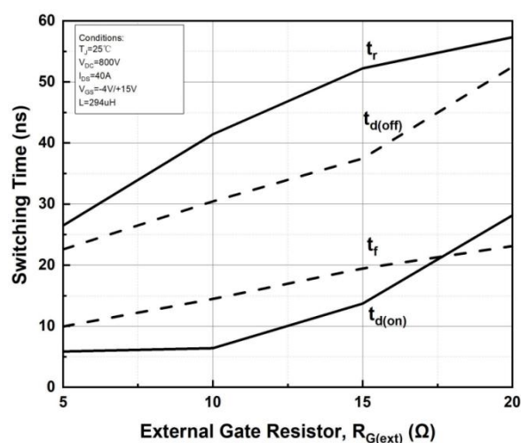
Figure 22. Switching Times vs. R_{G(\text{ext})}
