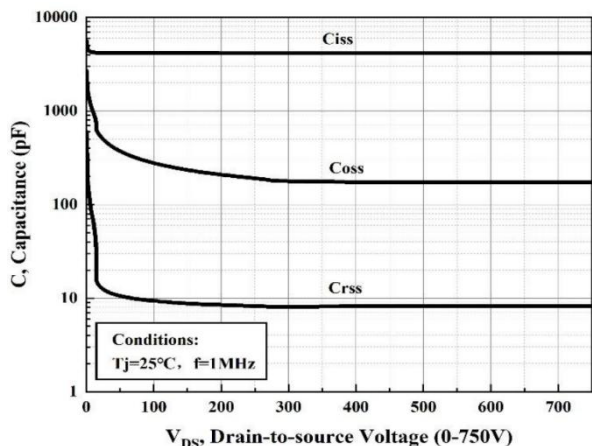
Figure 13. Capacitances vs. Drain Source Voltage (0-750V)
