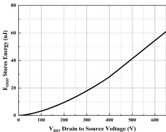
Figure 15. Output Capacitor Stored Energy
