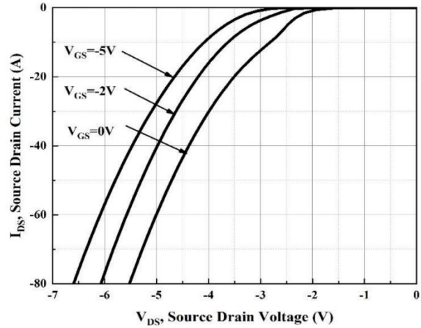
Figure 8. Body Diode Characteristic at Tj= 25 °C
