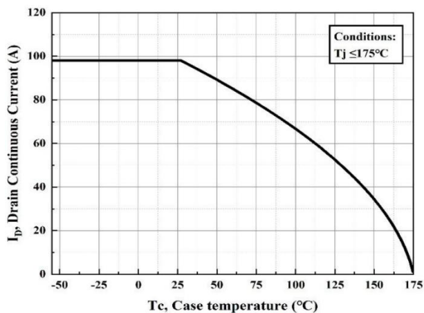
Figure 17. Continuous Drain Current Derating vs. Case Temperature
