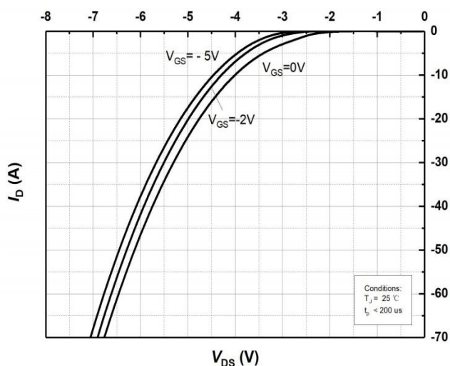
Figure 7. Body Diode Characteristics at Tj=25°C
