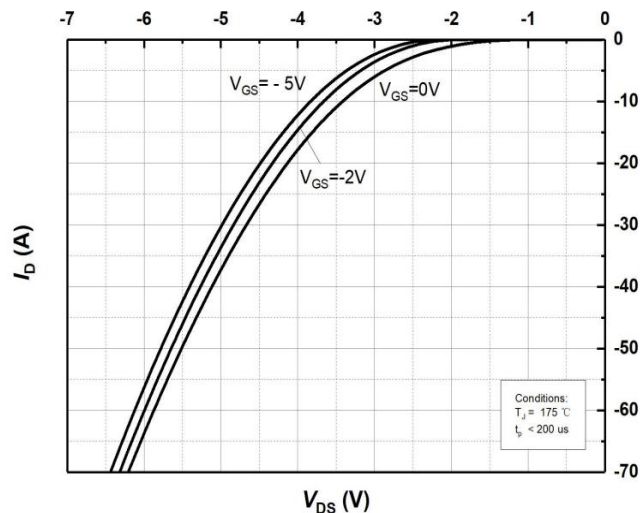
Figure 8. Body Diode Characteristics at Tj=175°C
