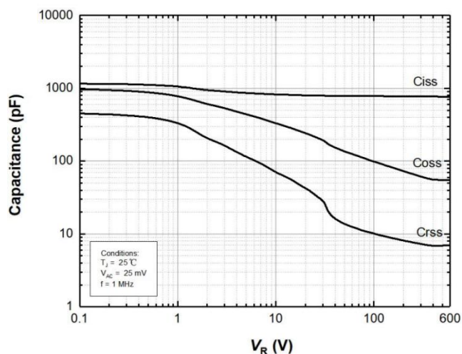
Figure 13. Capacitances vs. Drain-Source
