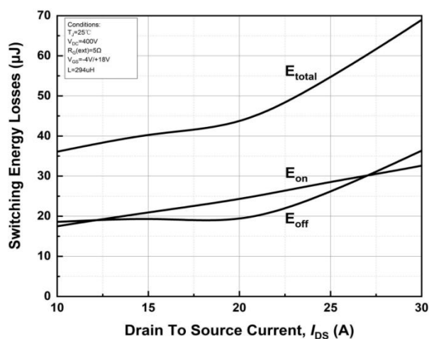
Figure 19. Clamped Inductive Switching Energy vs. Drain Current ( V_{DD} = 400V )
