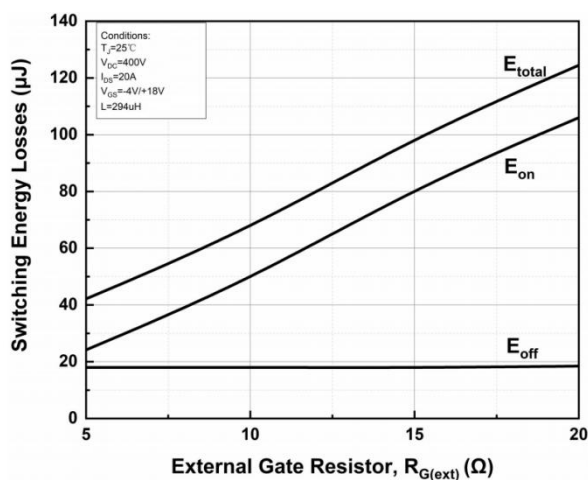
Figure 20. Clamped Inductive Switching Energy vs. R_{G(ext)}
