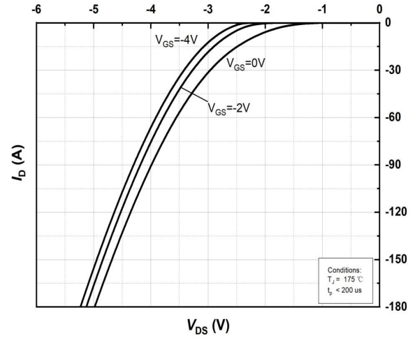
Figure 8. Body Diode Characteristics at Tj=175°C
