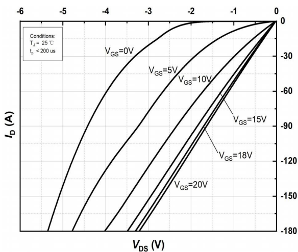
Figure 11. 3rd Quadrant Characteristic at Tj=25°C
