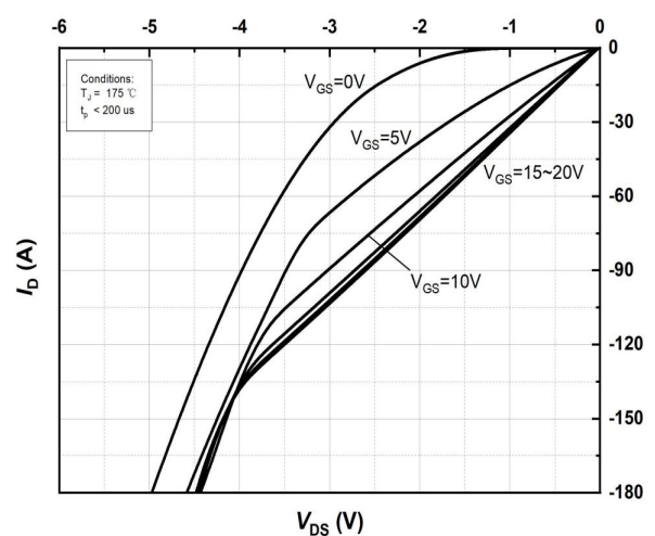
Figure 12. 3rd Quadrant Characteristic at Tj=175°C
