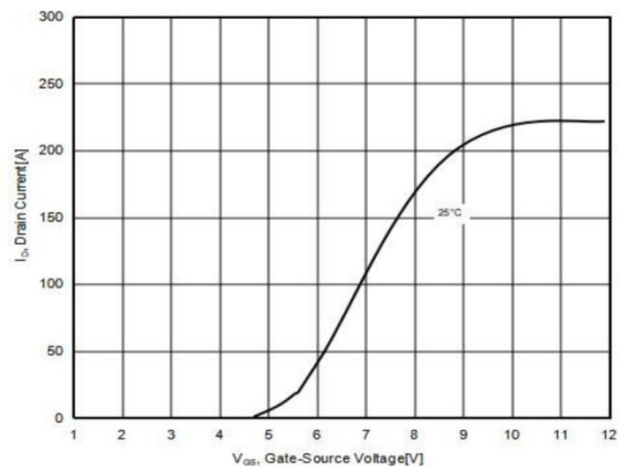
Figure4. Transfer characteristics
