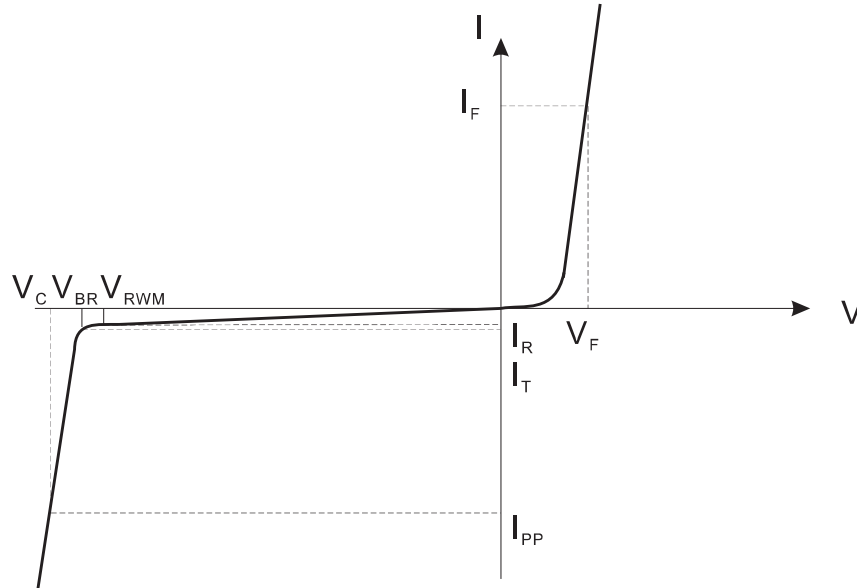
Uni-Directional TVS
