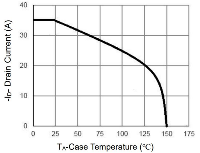
Figure 10 Current De-rating
