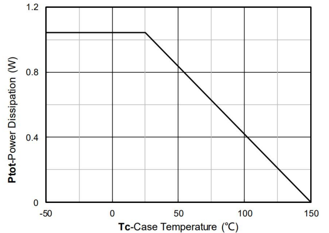
Figure 12. Power dissipation
