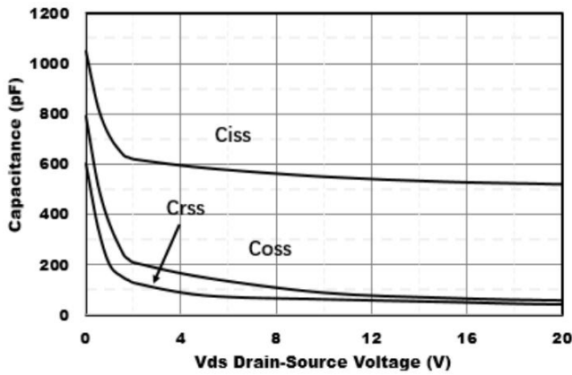
Figure3. Capacitance Characteristics
