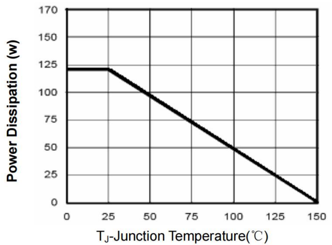
Figure 10 Power De-rating
